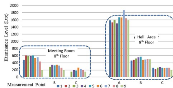
Figure 8. Comparison of illumination value in meeting rooms and hall area (8 th floor)
